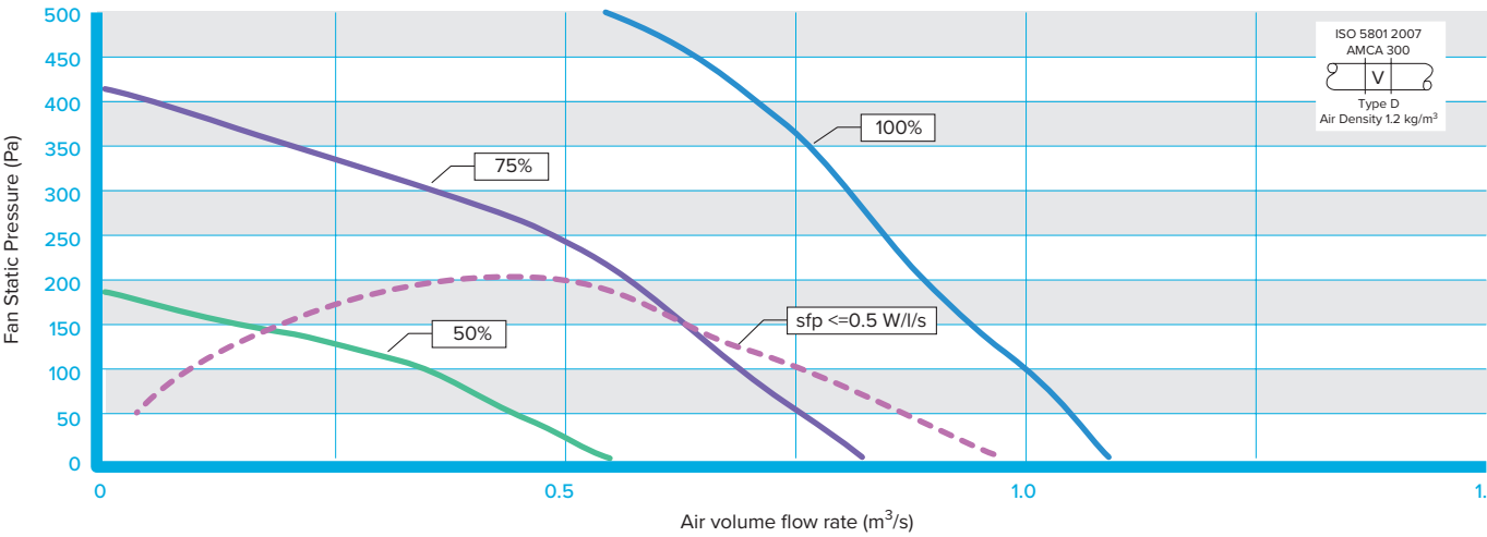
EXTRACT FAN SIZE DE7 - PERFORMANCE
